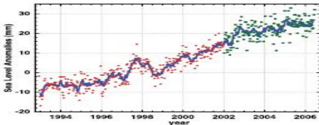
Figure 13.2. Variations in Global Mean Sea Level (in millimetres)
