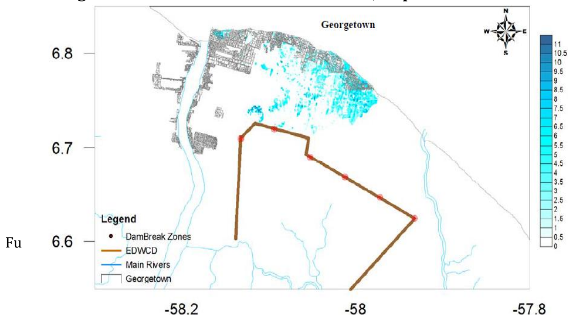
Figure 9. Dam Break Flood Hazard Result, Map for Zone 2 - EDWC
