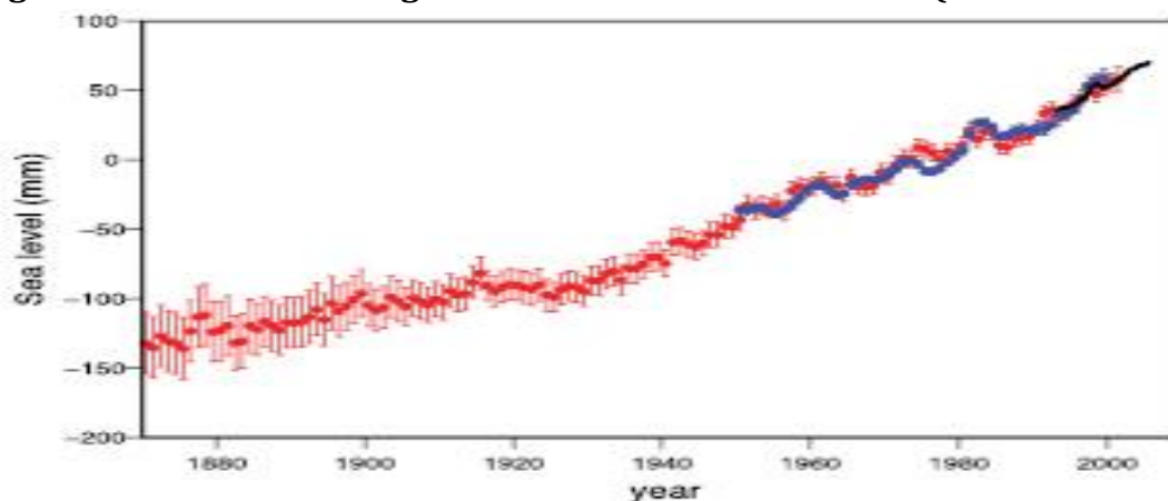
Figure 13.1. Annual Averages of the Global Mean Sea Level (in millimetres) 43
